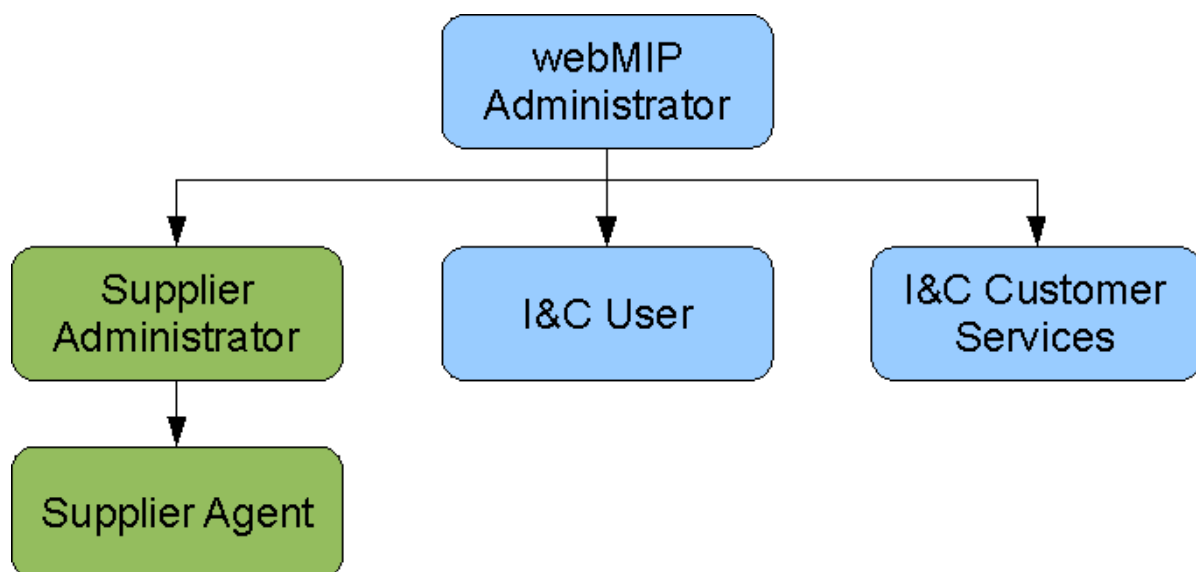
Illustration 1: User Role Hierarchy
